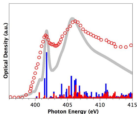
Figure 5. N 1s spectra of (C_{59}N)_2 azafullerene. Experimental STXM data in red circles, calculated spectrum using the Slater transition state in gray, projection of calculated spectrum into \pi^* (red) and \sigma^* (blue) components.
