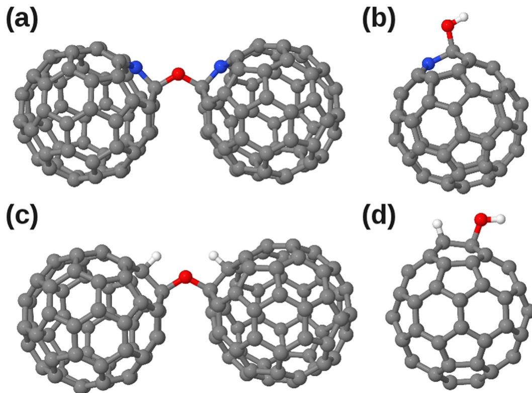
Figure 7. Structures of (a) C 59 N-O-C 59 N (b) C 59 N(OH), (c) C 60 H-O-C 60 H and (d) C 60 H(OH). Carbon atoms are shown in grey, oxygen in red, nitrogen in blue and hydrogen in white.
