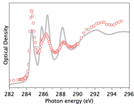
Figure 4. Carbon 1s spectrum of (C_{59}N)_2 . Experimental STXM data in red circles, calculated spectrum using the Slater transition state in gray is a weighted sum of individual atom spectra shown in Fig. 3.
