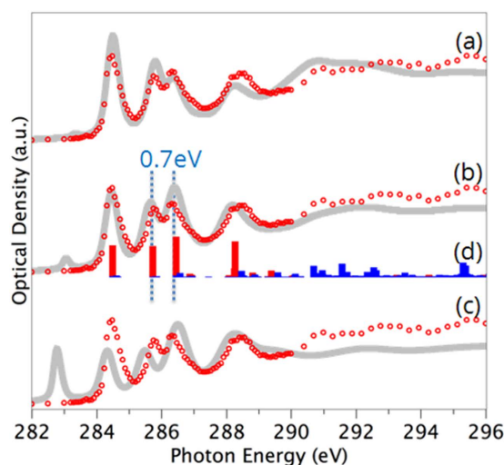
Figure 2. Carbon 1s spectrum of C_{60} . The experimental scanning transmission X-ray microscopy (STXM) data is plotted in red circles while the calculated spectra are gray lines. Calculations were performed with (a) full-core hole (final state), (b) half-core hole (Slater transition state) and (c) zero-core hole approximation (initial state). (d) Breakdown of calculated spectrum into \pi^* (red) and \sigma^* (blue) components.
