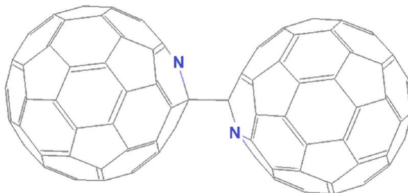
Figure 1. Structure of the azafullerene dimer ( C_{59}N ) 2 .
