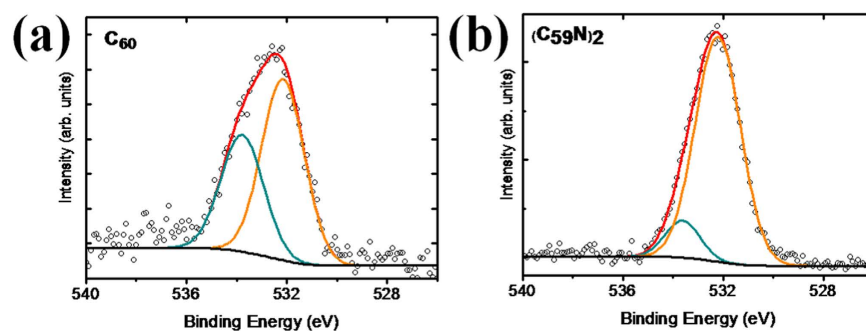
Figure 8. O 1s XPS signal for (a) C 60 and (b) (C 59 N) 2 powders.
