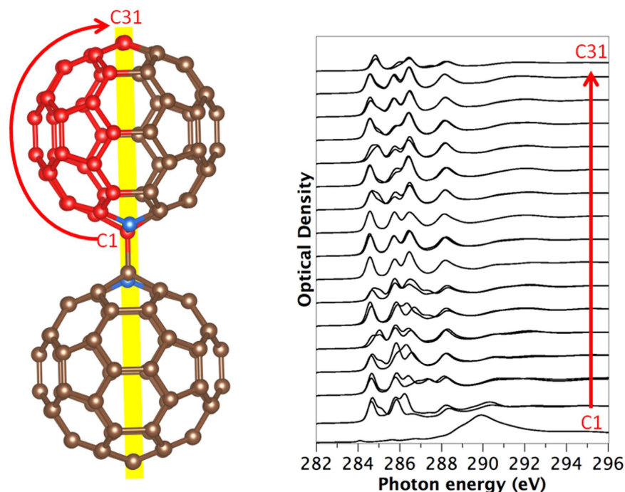
Figure 3. Calculated carbon 1s spectra using the Slater transition state, of (C_{59}N)_2 azafullerene for the symmetry inequivalent carbon atoms C_1 to C_{31} . Atom colors: Blue: Nitrogen, Red: inequivalent C atoms, Brown: other carbon atoms.
