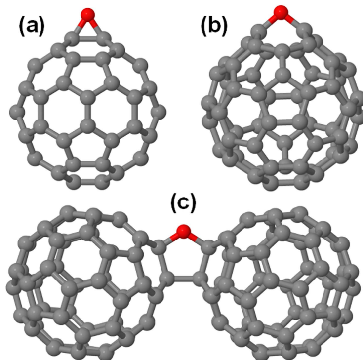
Figure 6. Stable oxygen-fullerene complexes: C_{60}O with oxygen in the (a) epoxide and (b) annulene configurations (c) ether-oxygen-bridged fullerene dimer C_{60}-O-C_{60} . Carbon atoms are shown in grey, oxygen in red.
