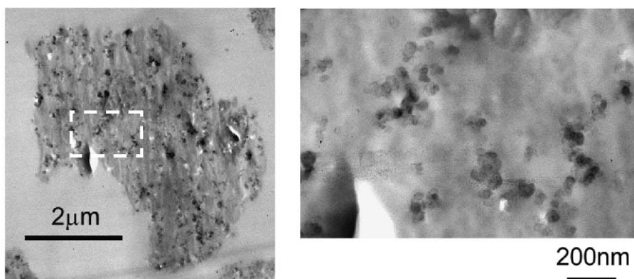
Fig. 1. TEM image of unstained pulverized toner.
