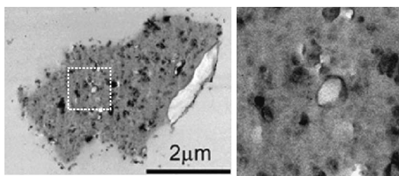
Fig. 2. TEM image of pulverized toner stained with RuO 4 vapor.
